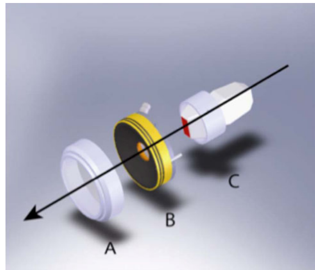
Fig. 1 Schematic diagram of the hand-held probe for ultrasound-guided repositioning of kidney stones: (a) the coupling standoff, (b) the focused annular array transducer, and (c) the ultrasound scan head. Coaxial arrangement of the probes places the focused ultrasound beam within the image plane
