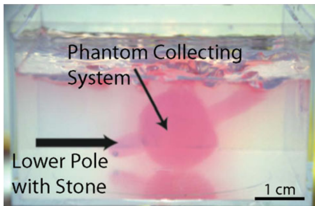
Fig. 3 Photograph of the kidney phantom with a simulated collecting system and lower pole. Artificial and human stones were placed dependently in the lower pole, and were repositioned to the collecting system using the ultrasound-guided therapy device. The hand-held source was in contact with the lower side of the phantom with its axis aimed vertically through the phantom. Stone repositioning in the transparent phantom was monitored concurrently with fluoroscopy, ultrasound imaging, and video photography
