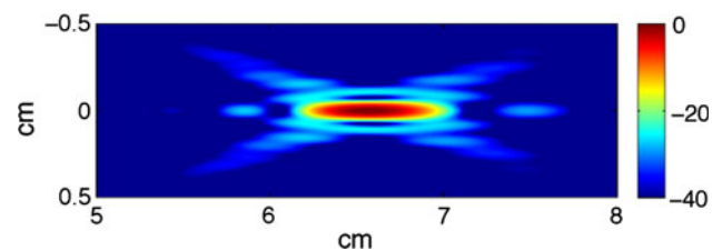
Fig. 2 Simulation of the focused ultrasound beam, from the annular array propagating from left to right, at a programed focal depth of 6.5 cm. The beam width was 0.6 and 1.1 cm at –6 and –20 dB, respectively. Scale in dB
